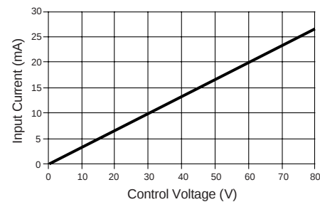
Figure 3d — Sxxxxx-22 relays
