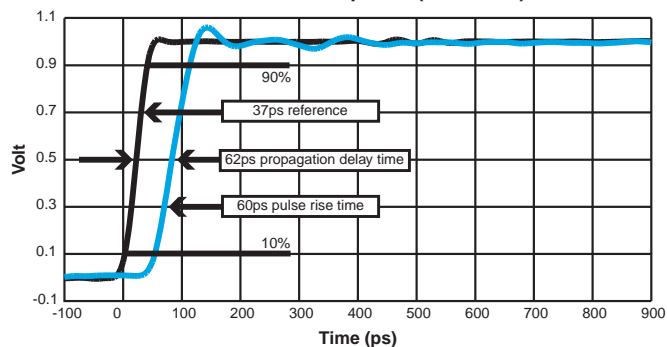
RF180 Time Response (RF Note 6)
