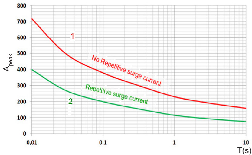
Figure 6c— 75A output
