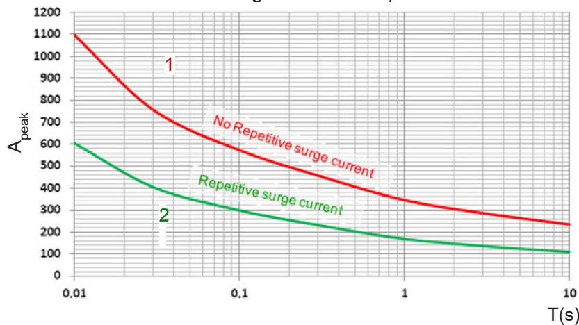
Figure 6c— 75A output
