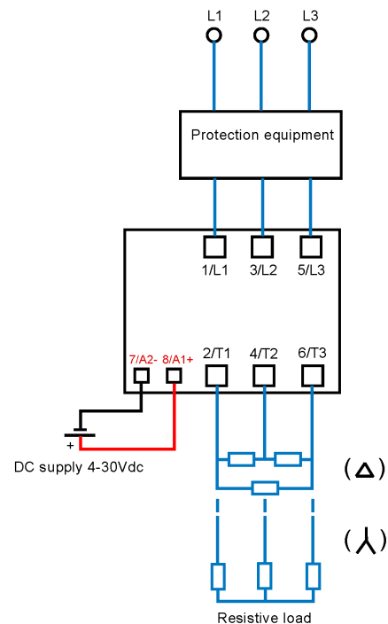
Figure 2 — Wiring Diagram
