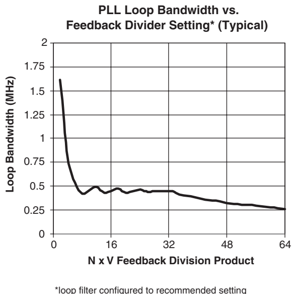
Figure 12. PLL Loop Bandwidth vs. Feedback Divider Setting (nominal)
