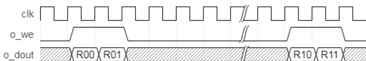
Figure 2.6. Result Interface Timing Diagram
