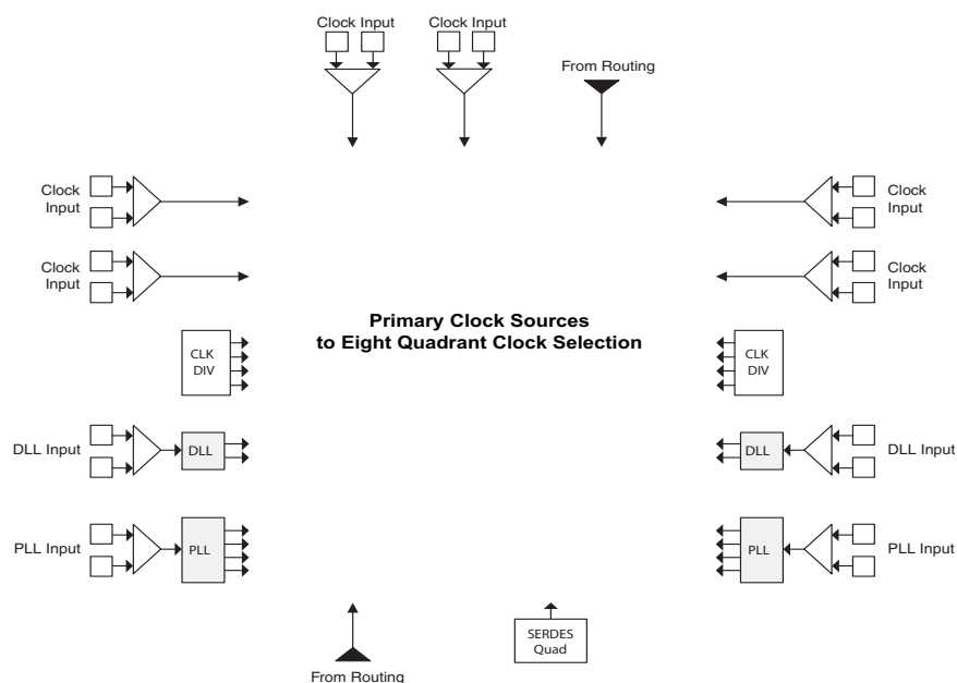
Figure 2-9. Primary Clock Sources for LA-LatticeECP3-17
