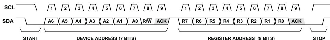
Figure 5-17. I 2 C Read Operation
