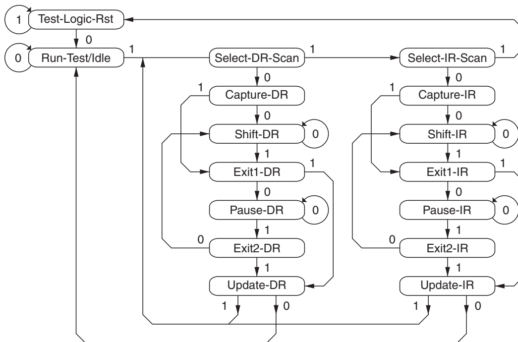
Figure 5-32. TAP States
