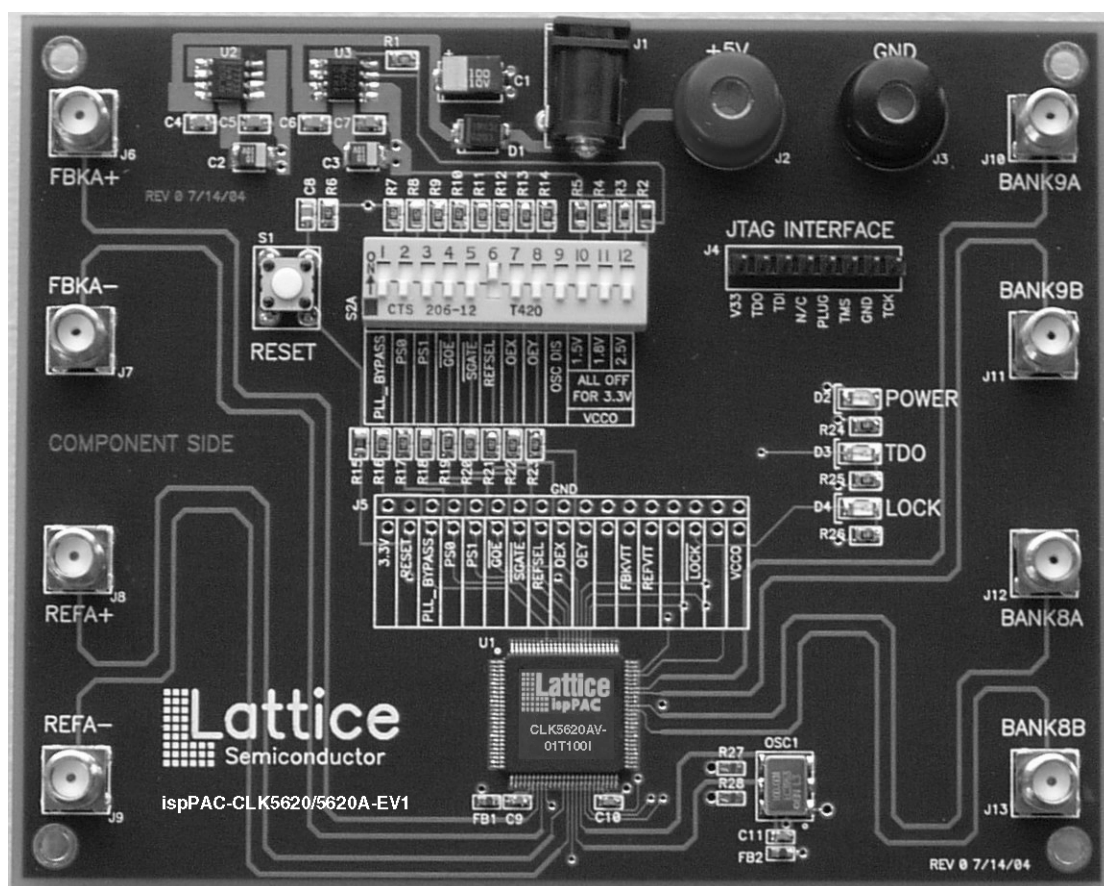
Figure 1. ispPAC-CLK5620A-EV1 Evaluation Board
