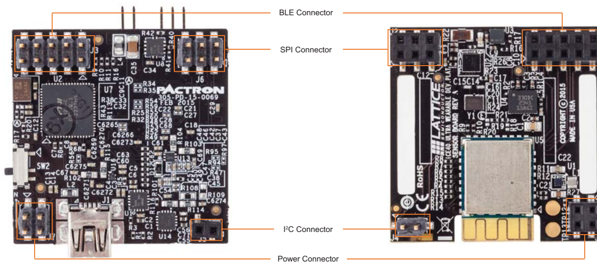
Figure 5. Headers
