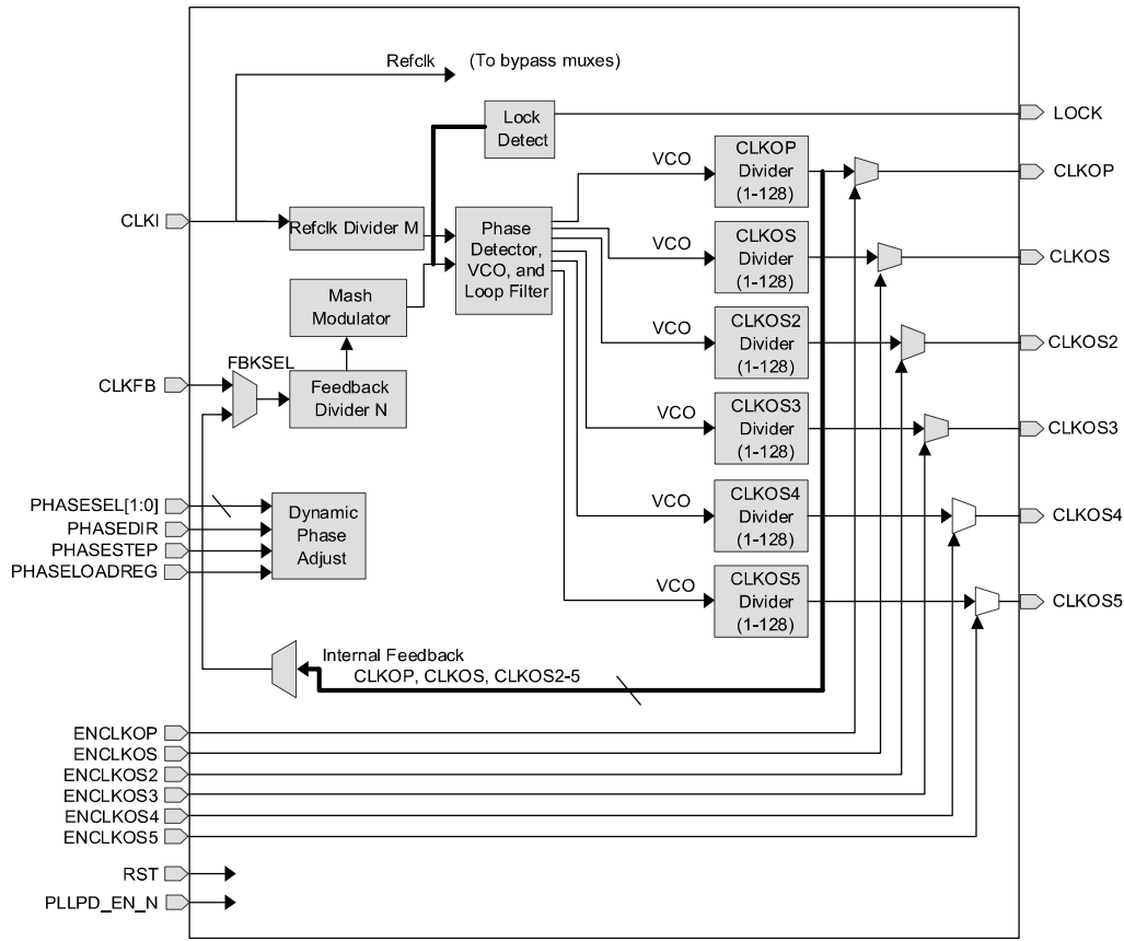
Figure 2.7. General Purpose PLL Diagram
