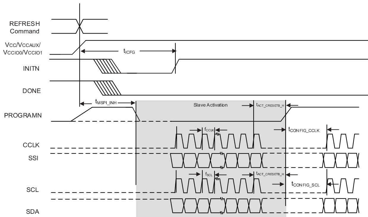
Figure 3.14. Slave SPI/I²C/I3C POR/REFRESH Timing
