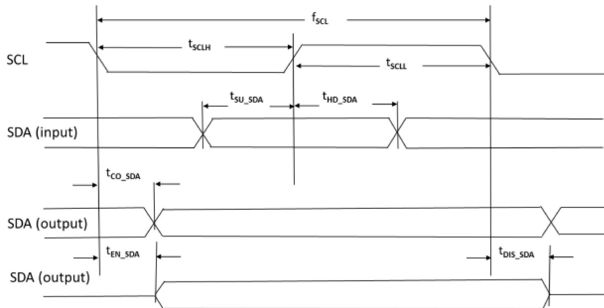
Figure 3.17. I²C /I³C Configuration Timing
