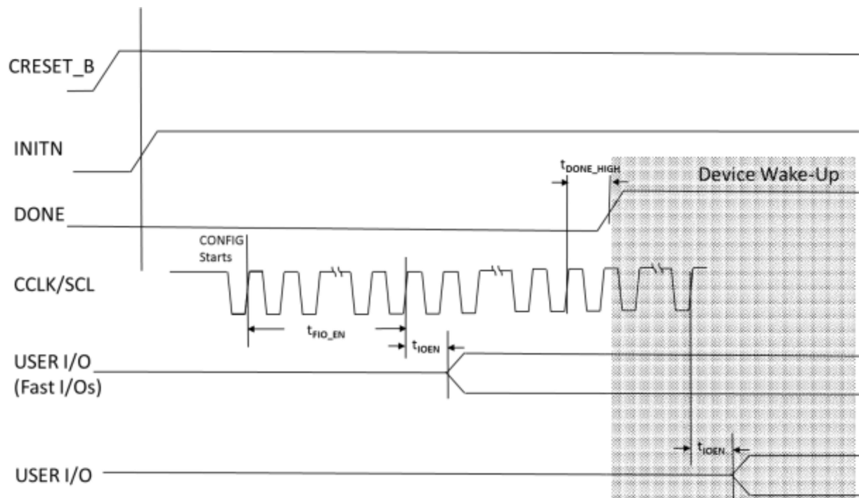
Figure 4.18. Slave SPI/I²C/I³C Wake-Up Timing
