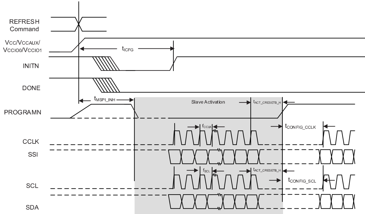
Figure 4.14. Slave SPI/I²C/I³C POR/REFRESH Timing
