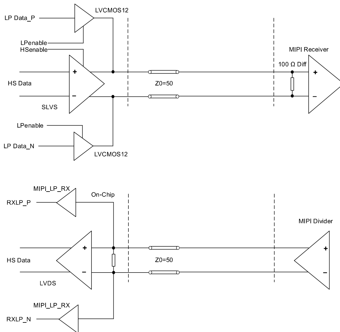
Figure 4.6. MIPI Interface
