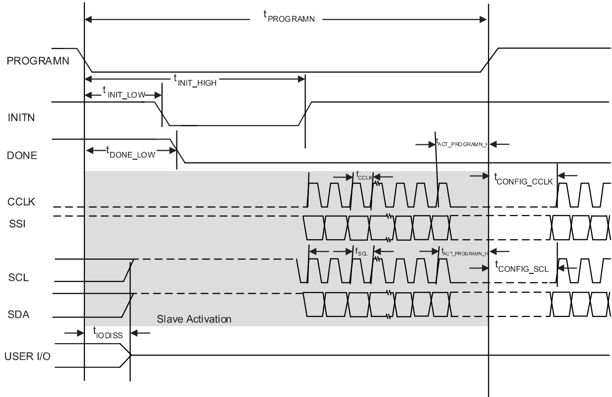
Figure 3.15. Slave SPI/I²C/I³C PROGRAMN Timing
