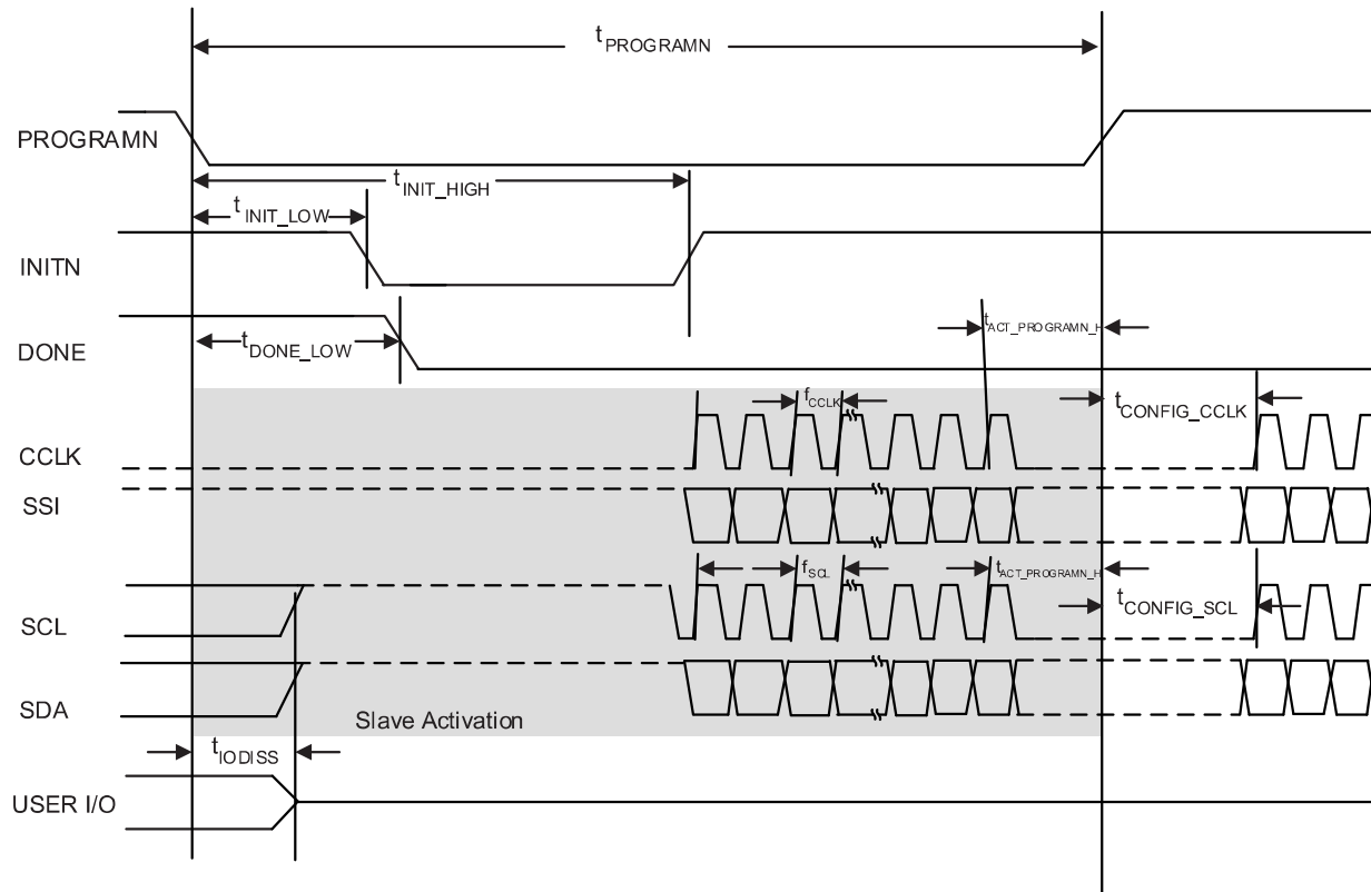
Figure 4.15. Slave SPI/I²C/I³C PROGRAMN Timing
