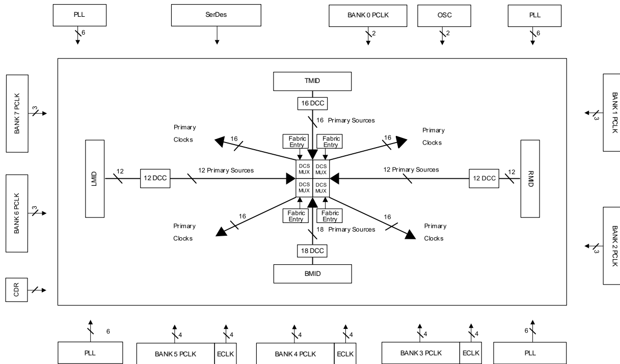
Figure 2.7. Clocking Network
