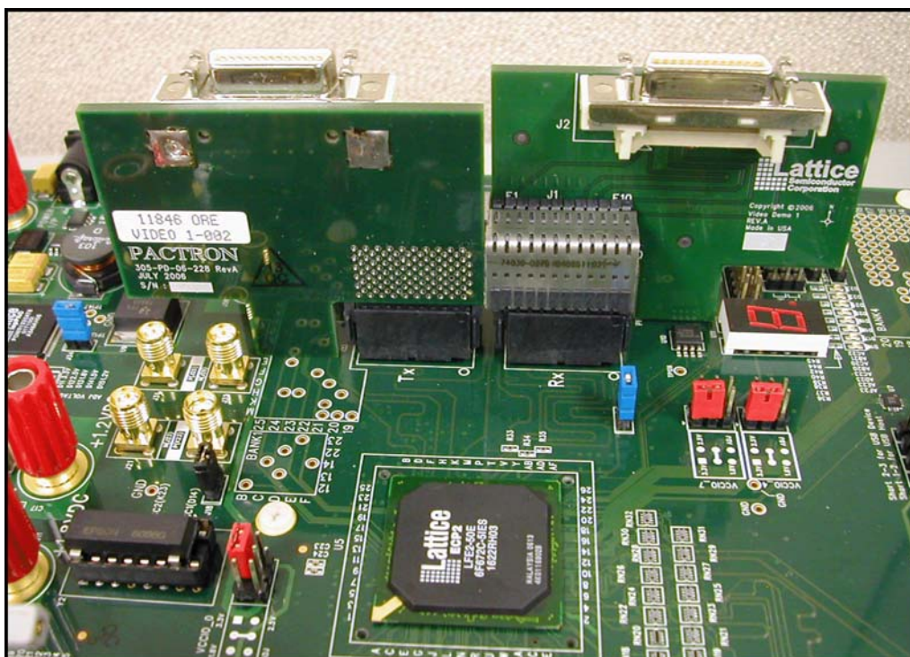
Figure 6. Proper Installation of Video Demo Boards #1 and #4 to the Lattice ECP2 Advanced Evaluation Board
