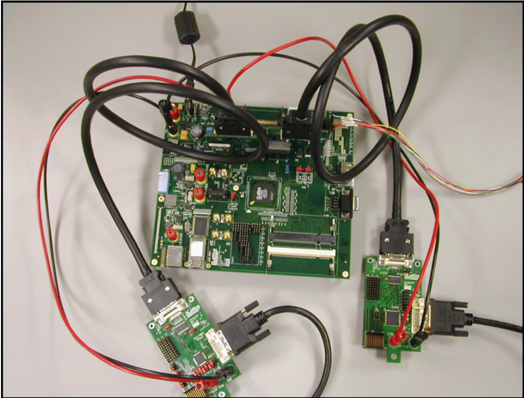
Figure 8. Power Cable Connections for Lattice 7:1 LVDS Video Demo Kit
