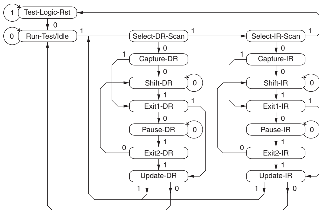
Figure 3-26. TAP States
