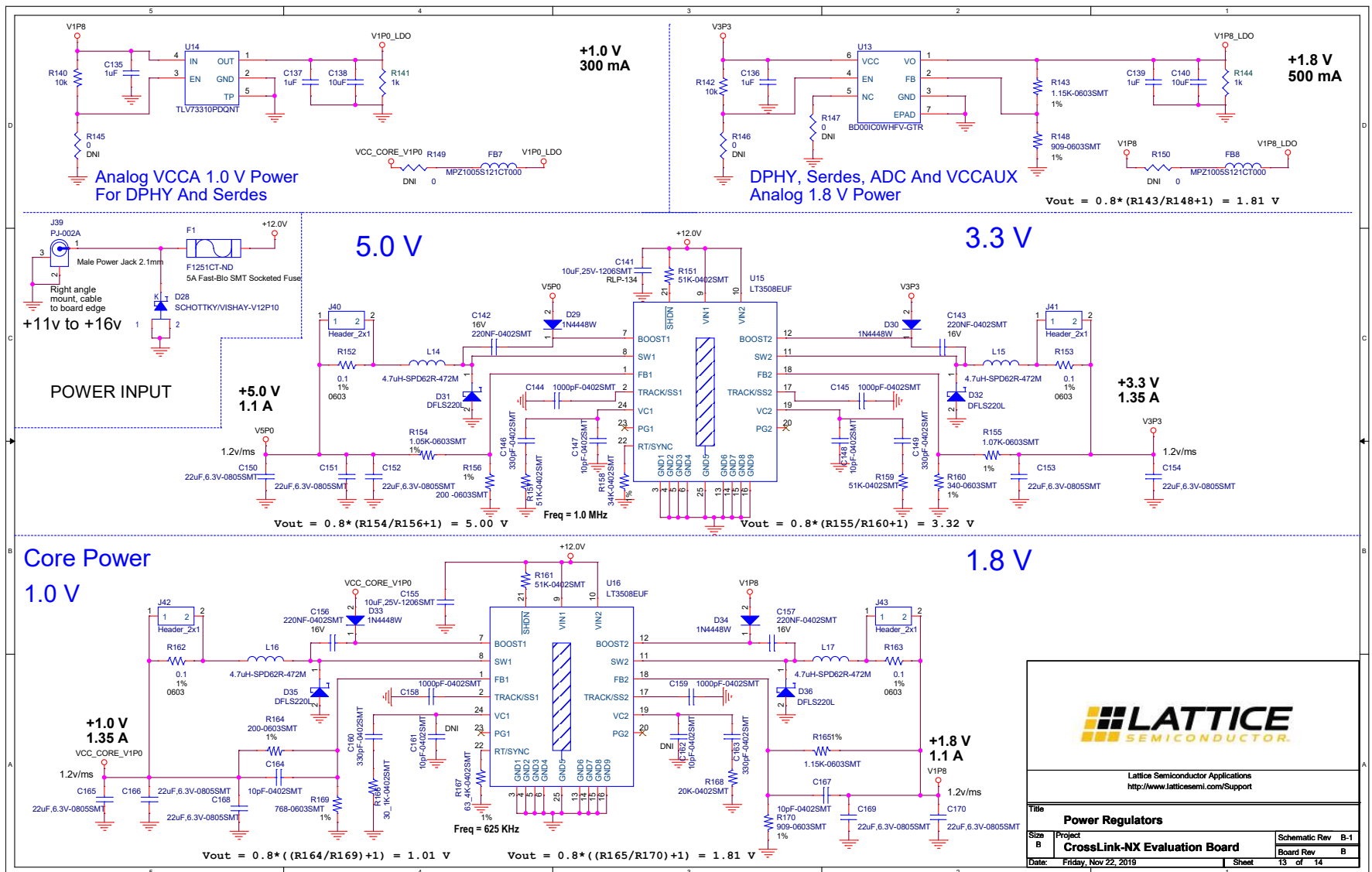
Figure A.13. Power Regulators
