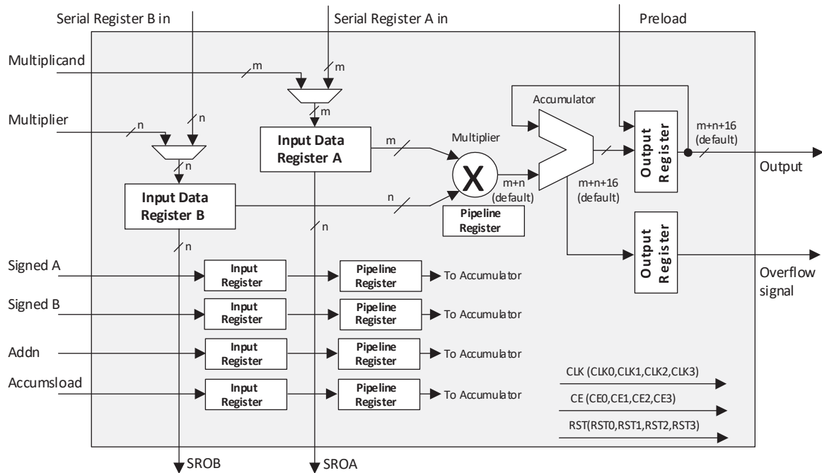
Figure 2.21. MAC sysDSP
