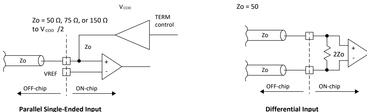
Figure 3.1. On-Chip Termination
