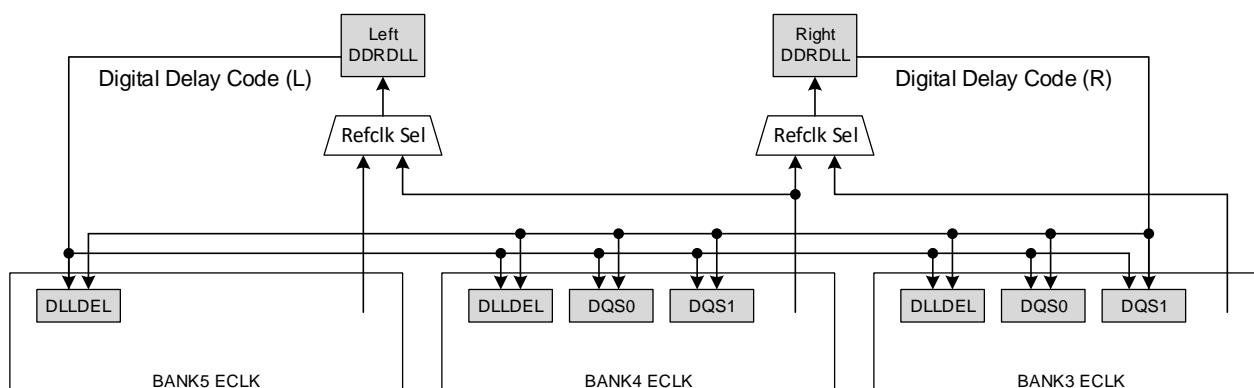
Figure 2.12. CrossLink-NX DDRDLL Architecture
