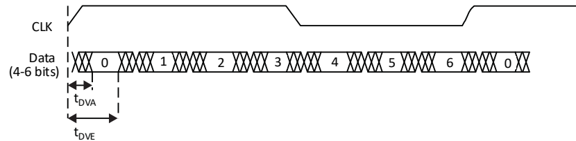
Figure 3.6.Receiver GDDR71_RX. Waveforms
