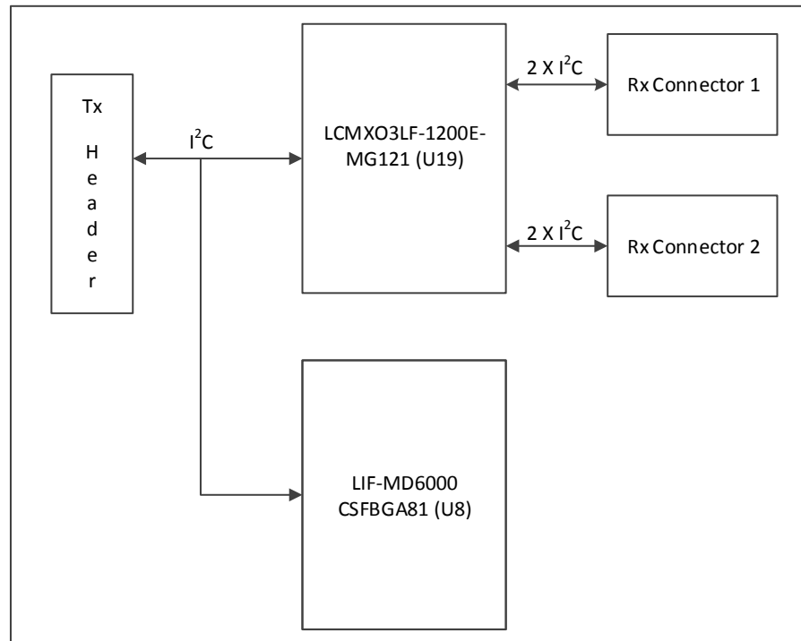
Figure 3.3. I 2 C Expander Block
