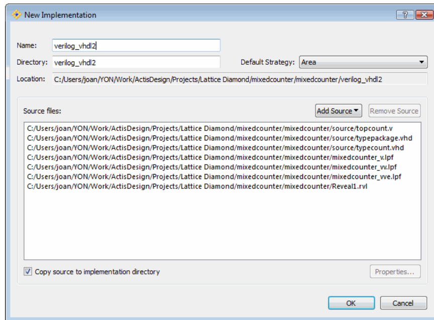
Figure 57: New Implementation
