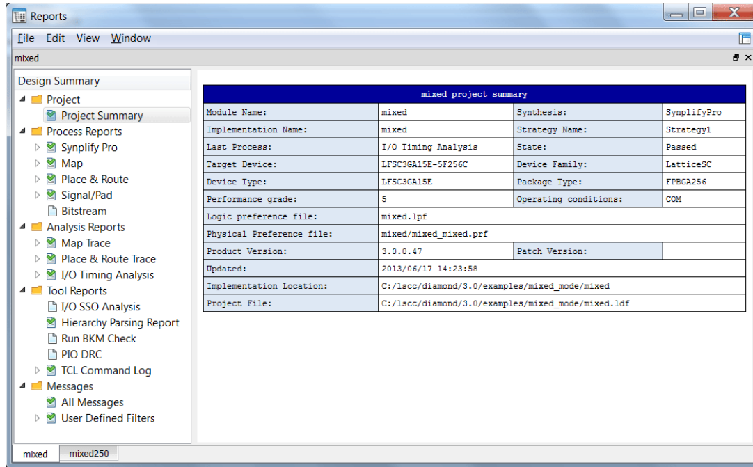
Figure 81: Reports View
