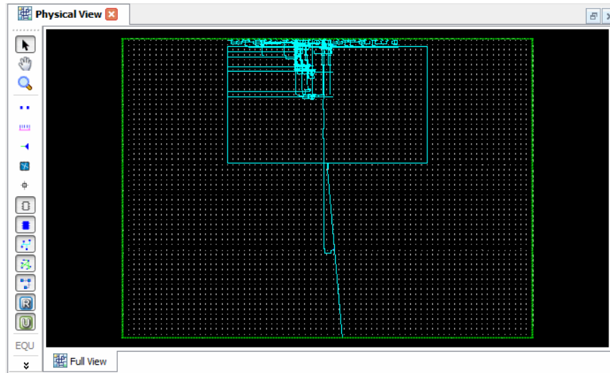
Figure 106: Physical View
