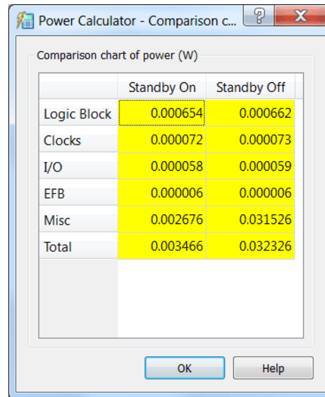
Figure 117: Standby Mode Comparison Chart
