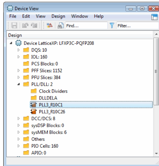
Figure 89: Device View
