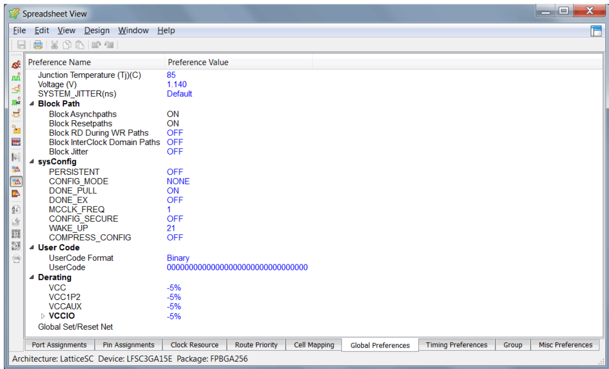
Figure 83: Spreadsheet View
