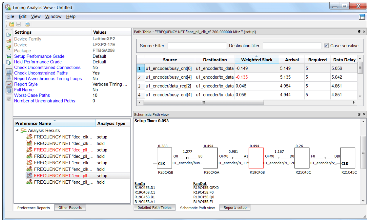
Figure 110: Timing Analysis Schematic Path View
