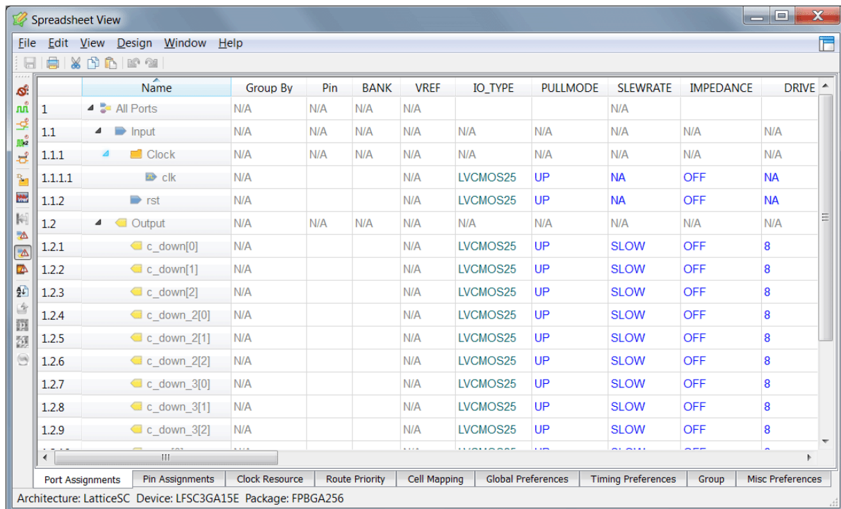
Figure 85: Spreadsheet View Port Assignments
