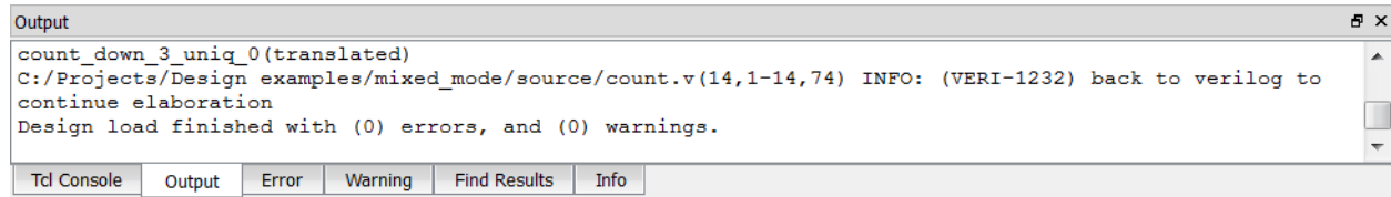
Figure 44: Output View
