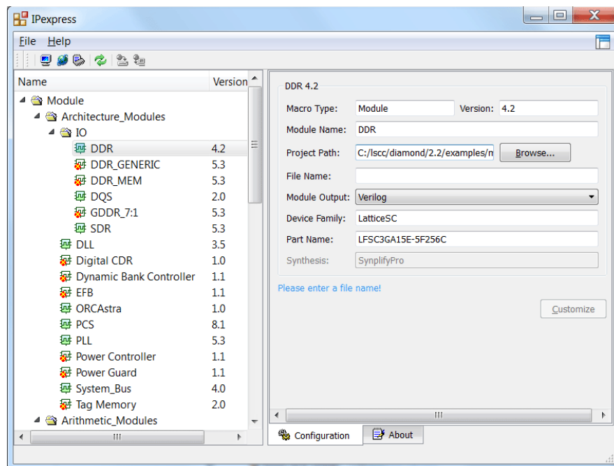
Figure 95: IPexpress
