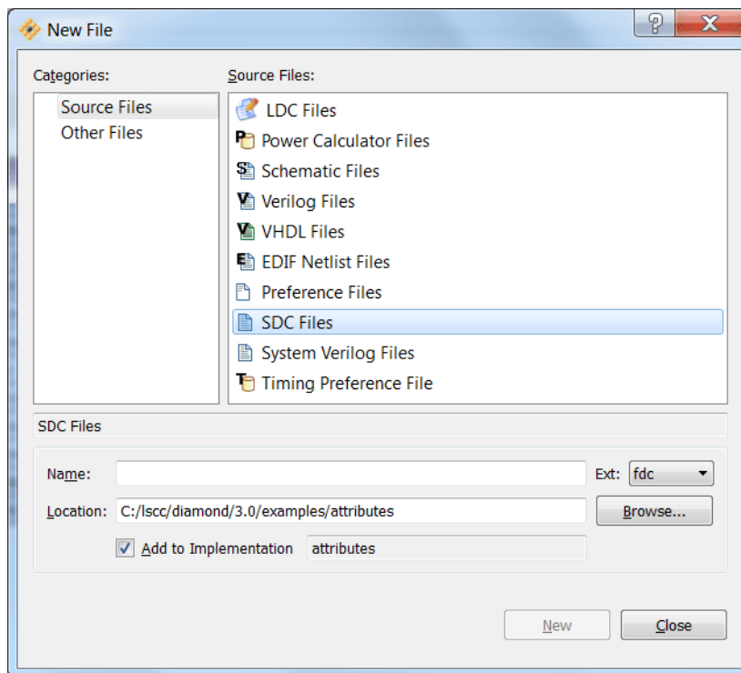
Figure 74: New Synthesis Constraint File
