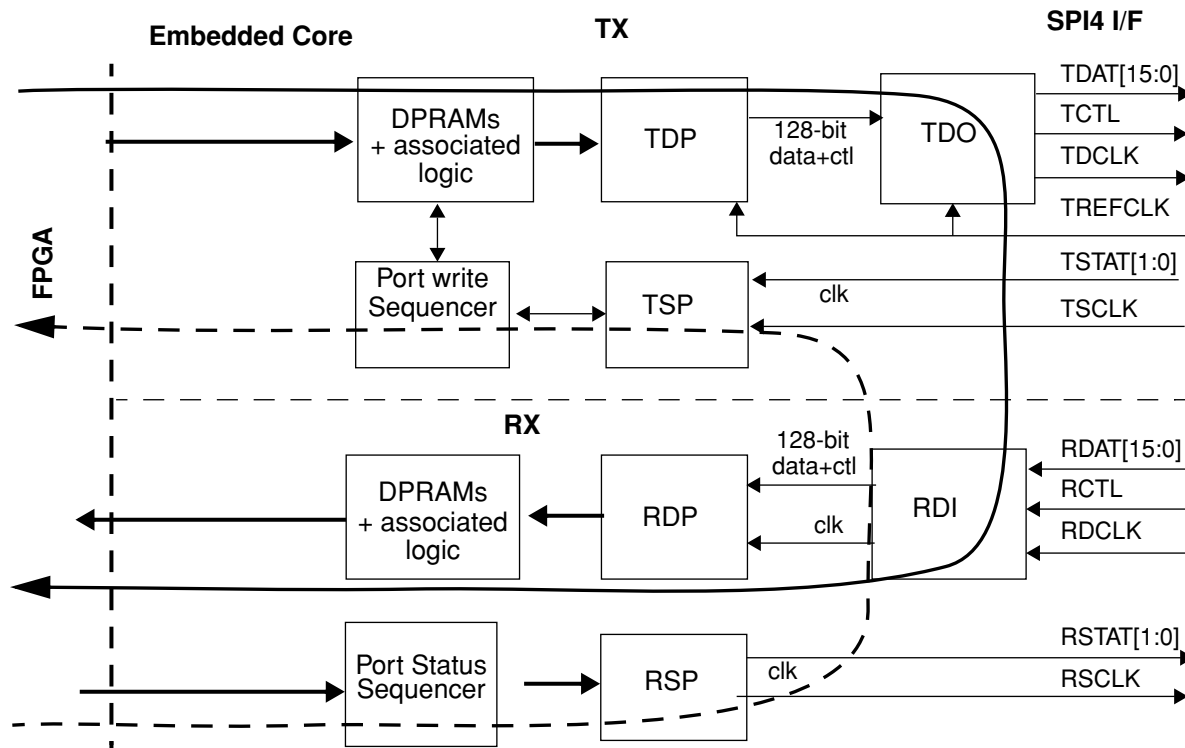
Figure 42. High-Speed Near End Loopback
