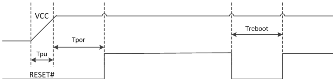
Figure 6 Reset Timing
