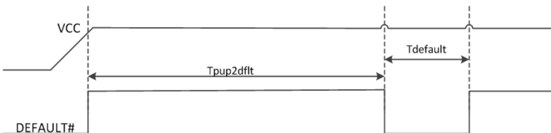
Figure 7 Reset to Defaults Timing
