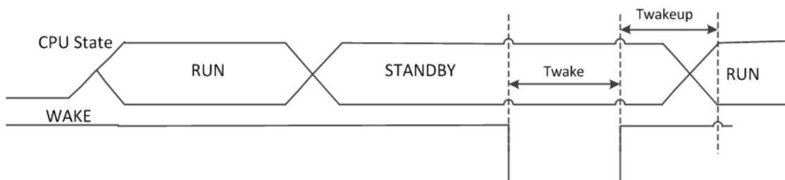
Figure 8 Wake Timing
