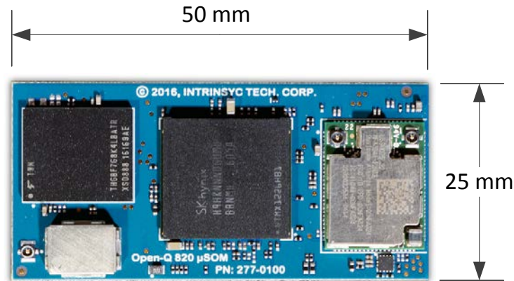
Figure 3 Open-Q 820 / 820Pro μSOM
