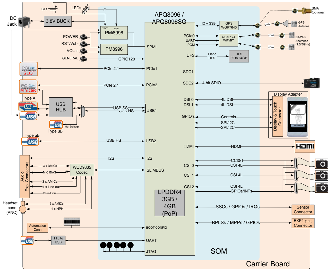
Figure 2 Open-Q 820 / 820Pro μSOM + Carrier Board Block Diagram
