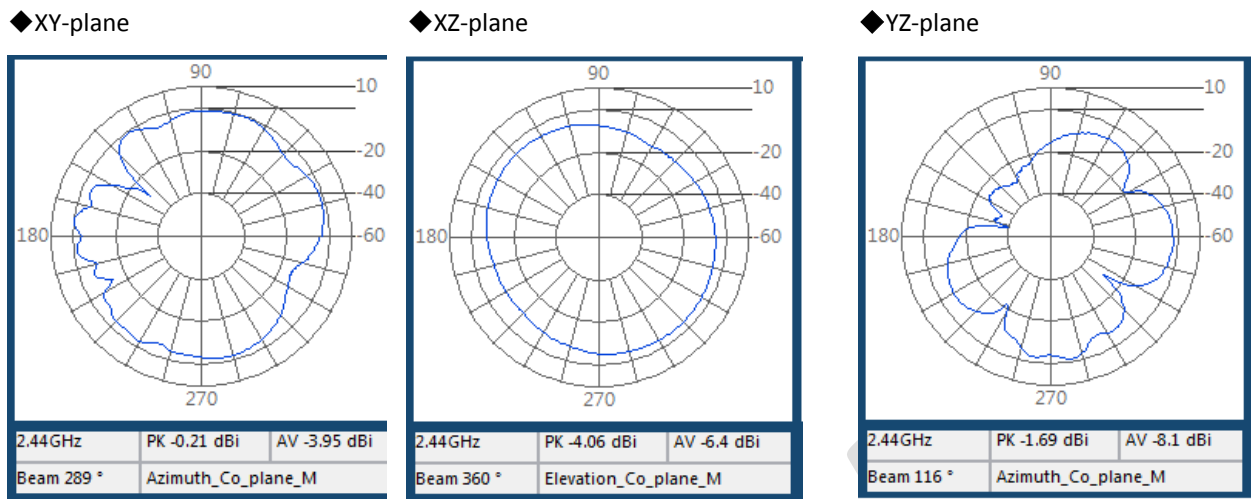
Figure 5: Trace antenna performance
