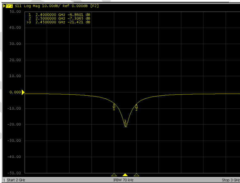
Figure 6: 453-00005 on-board PCB Trace antenna performance (Antenna Gain, efficiency and S11 (whilst 453-00005 module on DVK-BL652-xx development board)
