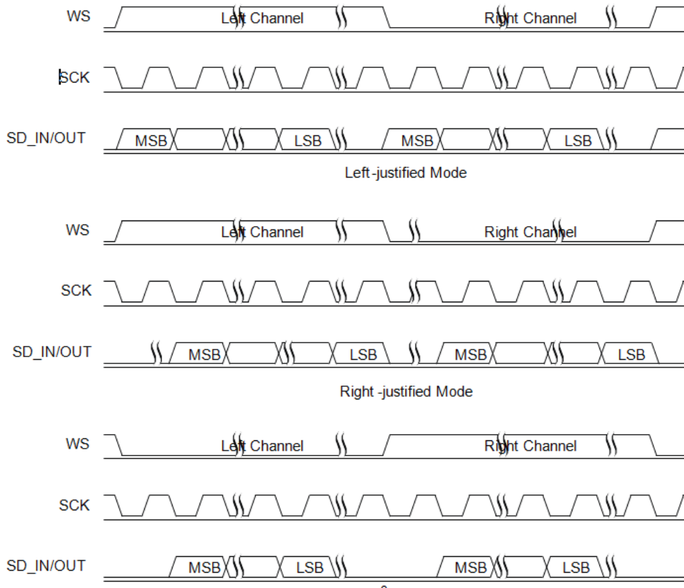
Figure 13: PCM configuration
