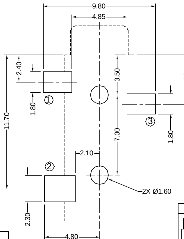
Recommended PCB Layout (Top View)
