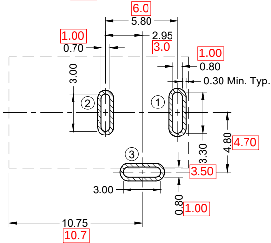
Recommended PCB Layout (Top View) Ref. Tol. \pm 0.05
