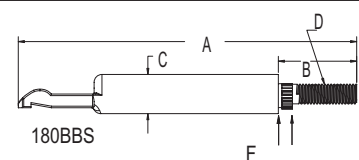
Bus Bar
