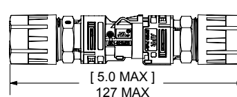
SK1-021M05 & SK6-021M05 (mated)
