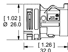
Male Receptacle SK1-021M05
