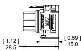
Female Plug SK6-021M05
