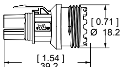
Female Plug SK6-019M03
