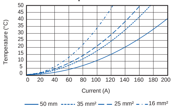
EBC 160 Temperature Rise
