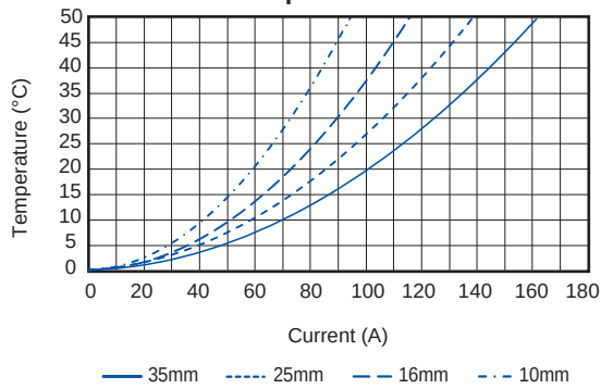
EBC 80 Temperature Rise
