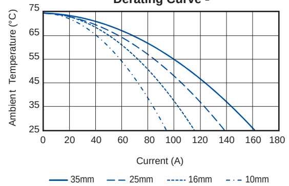
EBC 80 Derating Curve 1
