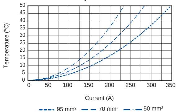
EBC 320 Temperature Rise
