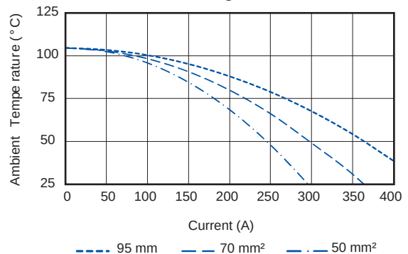
EBC 320 Derating Curve 1
