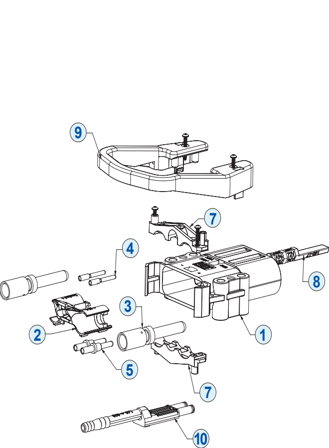
Male Connector
