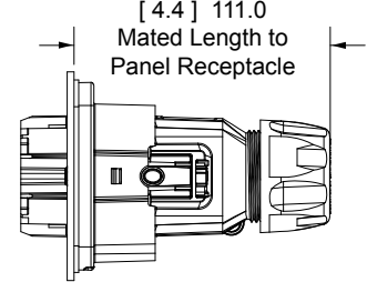
Mated View
