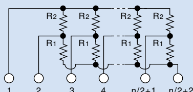
R circuit
