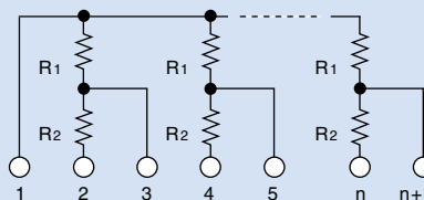
T circuit
