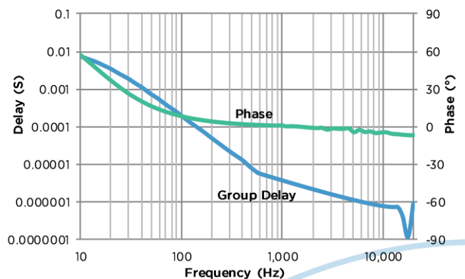
Figure 5: Typical Phase Response and Group Delay
