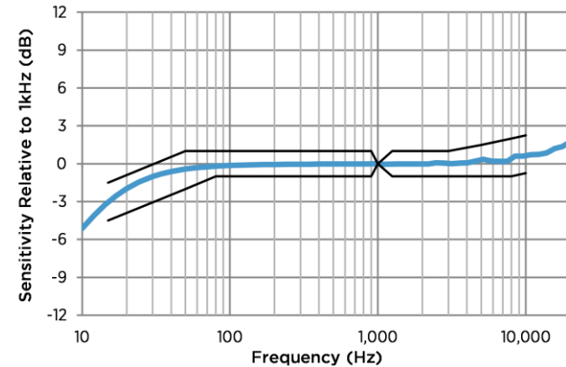
Figure 3: Typical Free Field Magnitude Response and Masks
