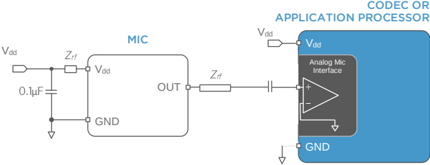
Figure 1: Typical Single-Ended Application Circuit
