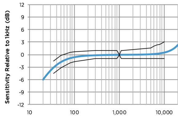
Figure 3: Typical Free Field Magnitude Response and Masks
