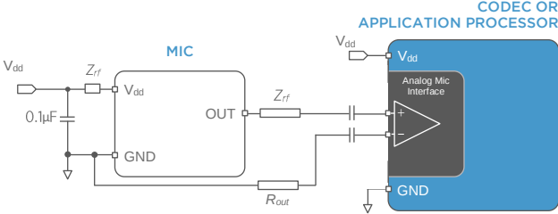
Figure 2 Typical Differential Mode Application Circuit
