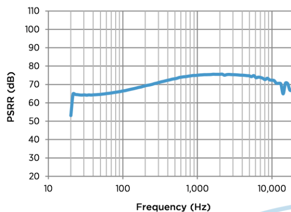
Figure 10: Typical PSRR
