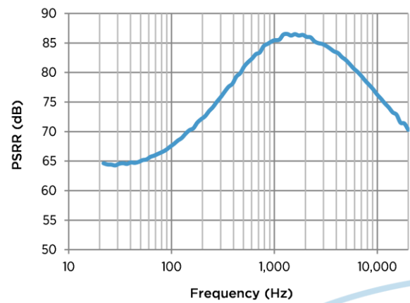
Figure 10: Typical PSRR
