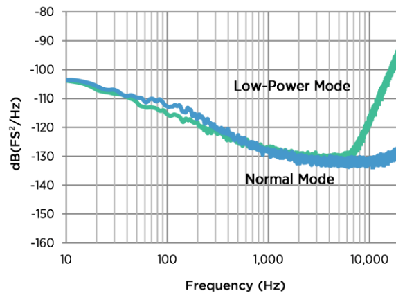
Figure 13: Typical PSRR
