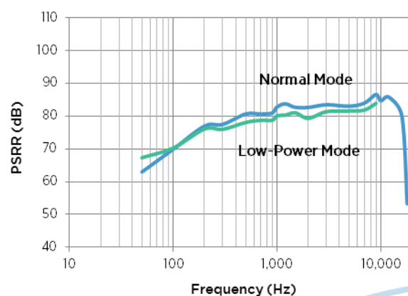
Figure 12: Typical PSRR
