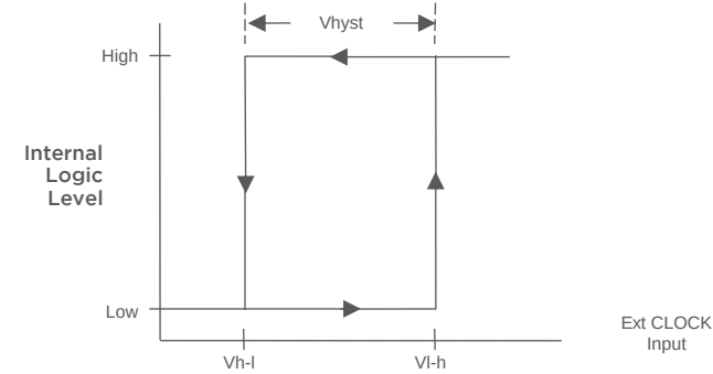
C Figure 2: Hysteresis Diagram
