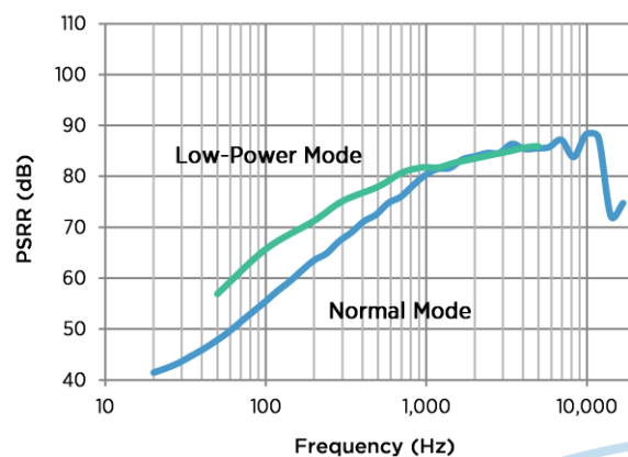
Figure 13: Typical PSRR
