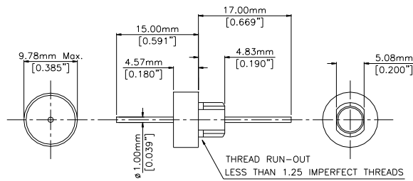
Dimensions mm (inches)
