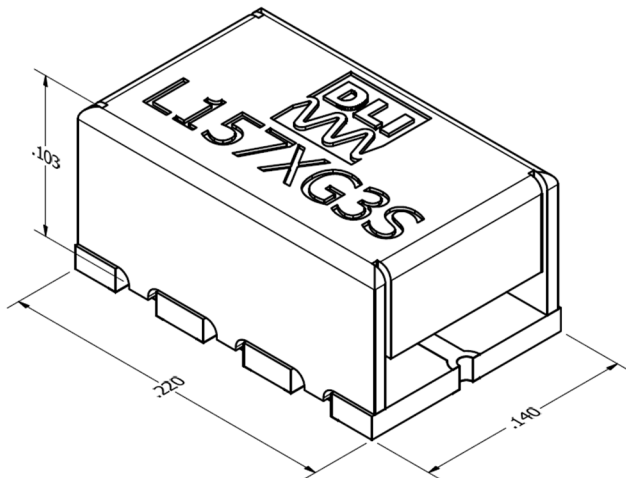
Isometric View
