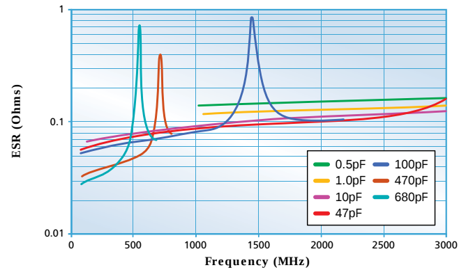
Q(MS) Series - ESR vs. Frequency - Case size 1111
