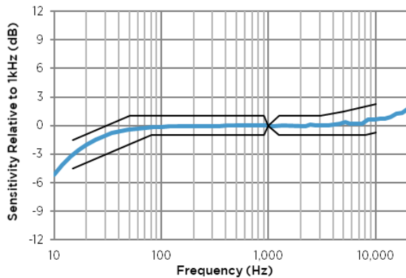
Figure 3: Typical Free Field Magnitude and Masks
