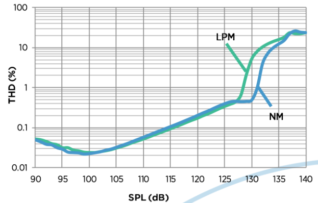
Figure 5: Typical THD vs SPL
