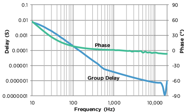
Figure 4: Typical Phase and Group Delay
