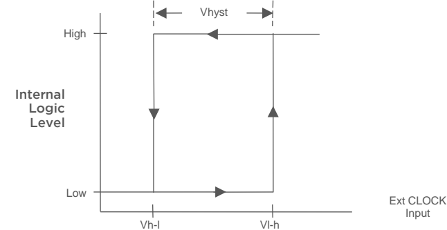
Figure 2: Hysteresis Diagram
