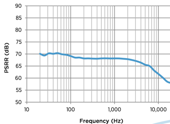
Figure 9: Typical PSRR
