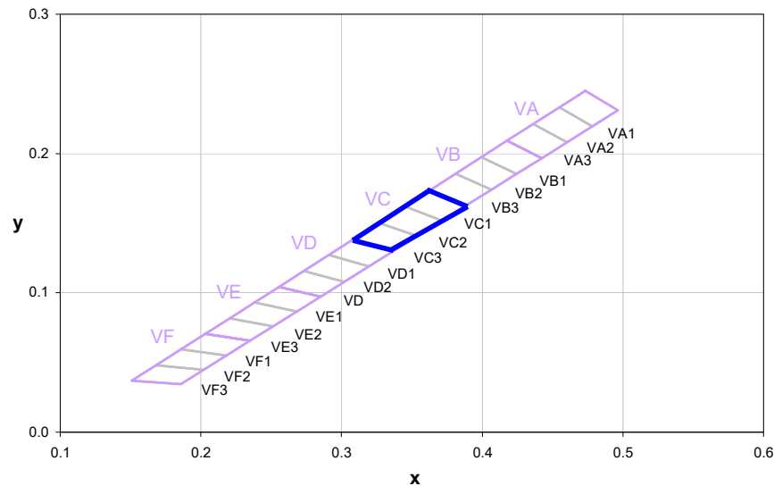
CIE CHROMATICITY DIAGRAM
