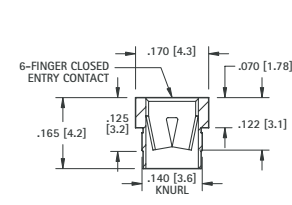
.084 (2.13) - .102 (2.6) PIN - PRESS-FIT
