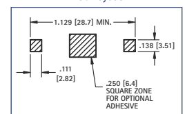
Pad Layout
