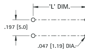
Mounting Detail
