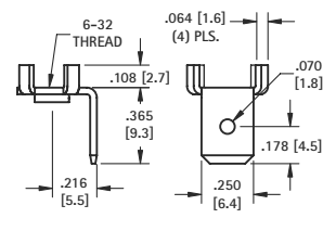
Mounting Detail
