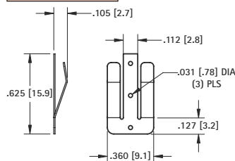
DWG. 2 MATERIAL: .010 (.25) Phosphor Bronze
