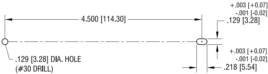
SUGGESTED MOUNTING DETAIL
