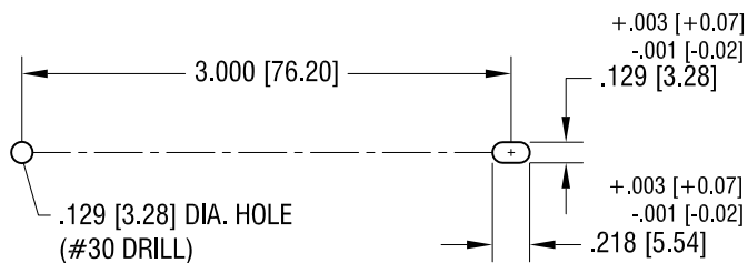
SUGGESTED MOUNTING DETAIL
